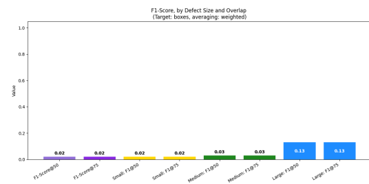
Figure 24: F1-Score Testing
