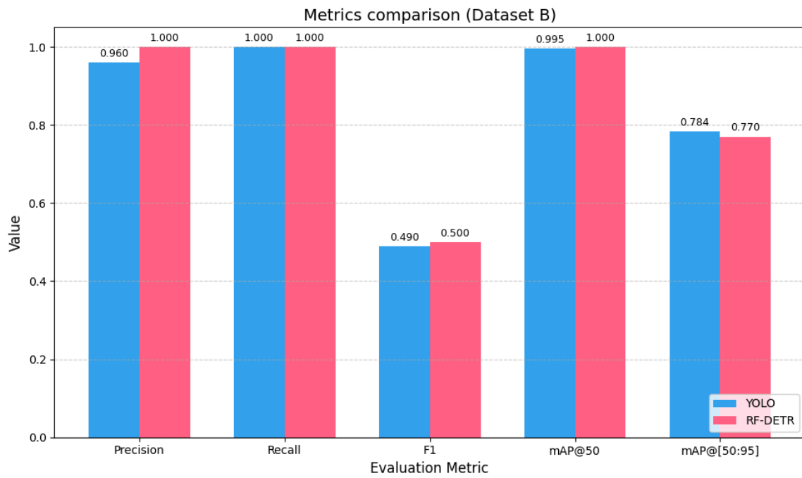
Figure 11: Visualization of Results for Dataset B
