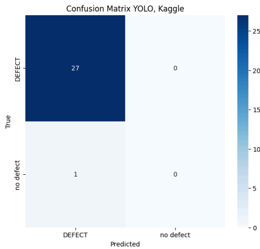
Figure 9: Confusion Matrix YOLO Dataset
