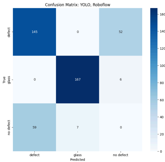
Figure 6: Confusion Matrix YOLO Dataset
