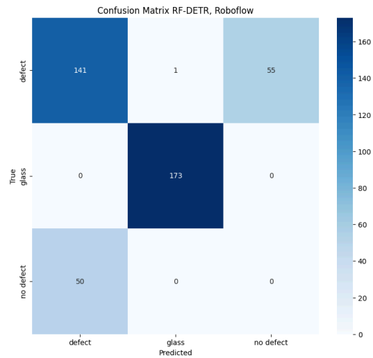
Figure 7: Confusion Matrix RF-DETR
