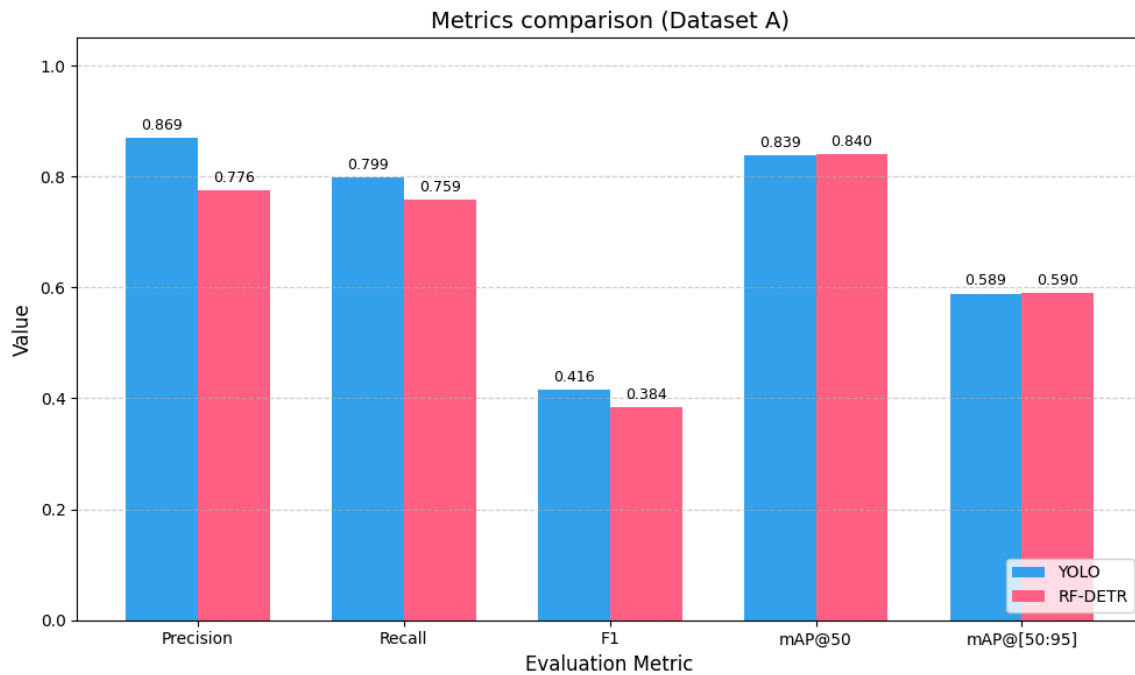
Figure 8: Visualization of Results for Dataset A
