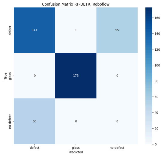
Figure 11: Confusion Matrix RF-DETR Dataset A
