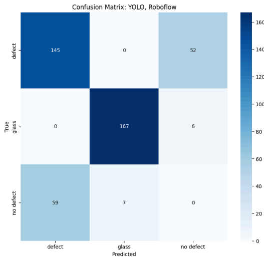
Figure 10: Confusion Matrix YOLO Dataset A
