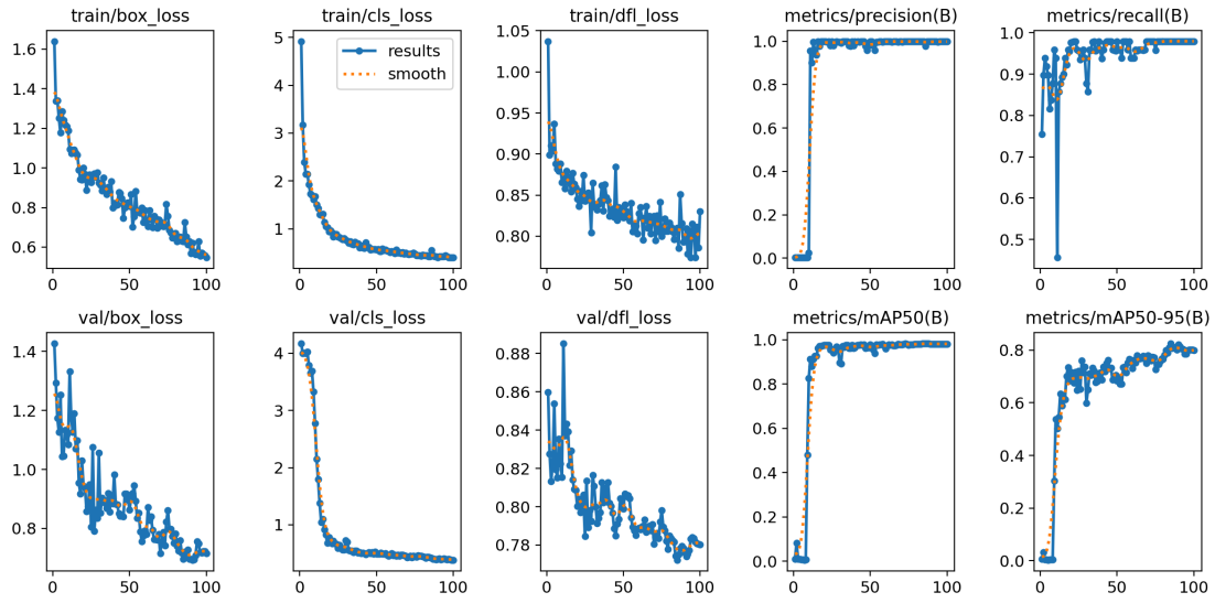
Figure 5: Training results
