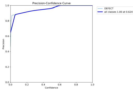
Figure 6: Precision Testing
