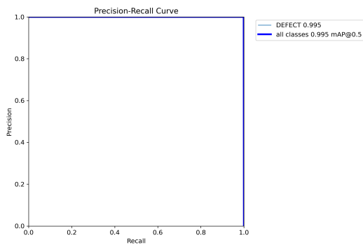
Figure 8: Precision/Recall Testing
