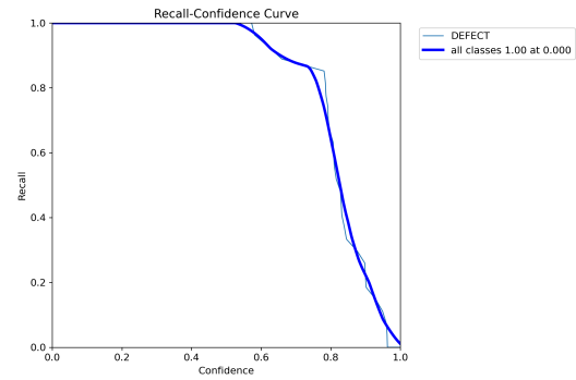
Figure 7: Recall Testing
