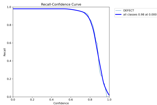
Figure 3: Recall Training
