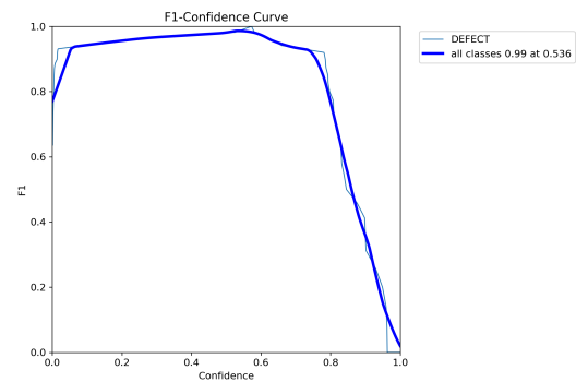
Figure 9: F1-Score Testing
