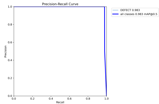
Figure 2: Precision/Recall Training
