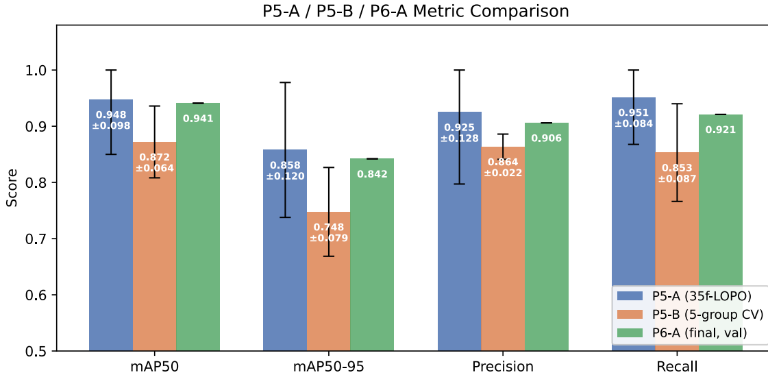
Figure 16: Performance comparison across P5-A (35-fold LOPO, test), P5-B (5-group CV, test), and P6-A (final model, val). Error bars show std across folds, clipped at 1.0. P6-A is a single training run with no held-out test set.
