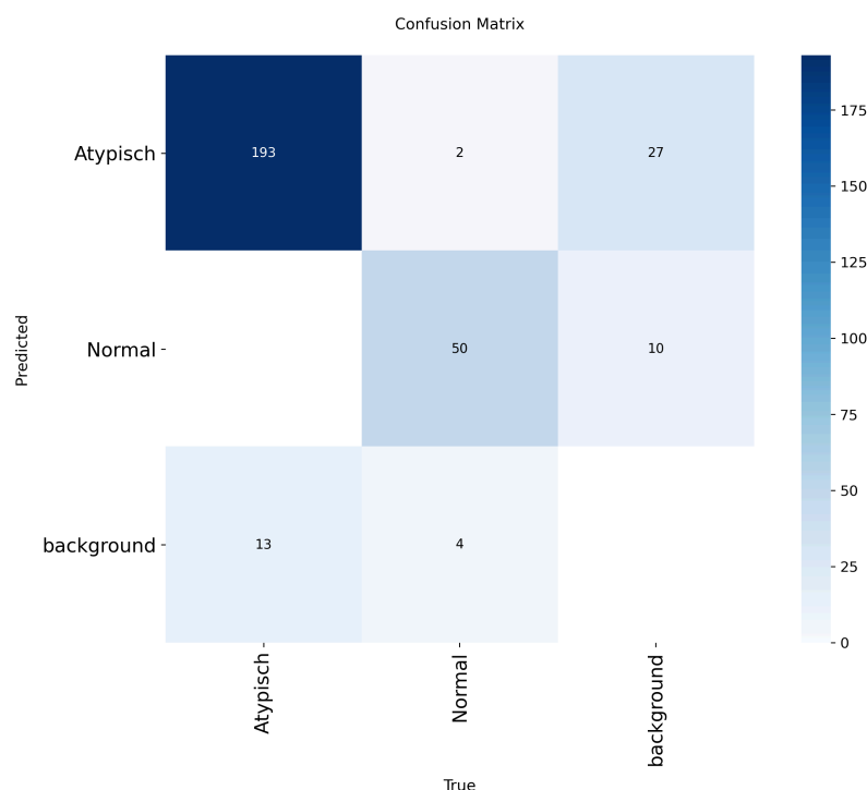
Figure 19: Confusion matrix for P6-A raw numbers.
