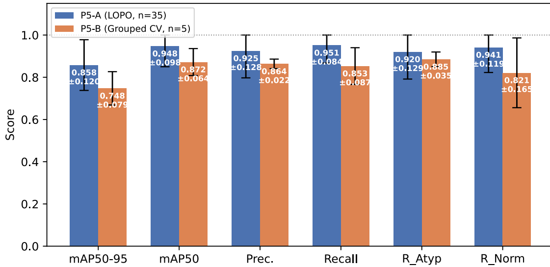
Figure 15: Metric comparison between P5-A (35-fold LOPO) and P5-B (grouped 5-fold CV). Error bars represent \pm 1 standard deviation across folds. R_AtYP and R_Norm for P5-A are computed over the 20 and 29 folds respectively where the class was present in the test set.
