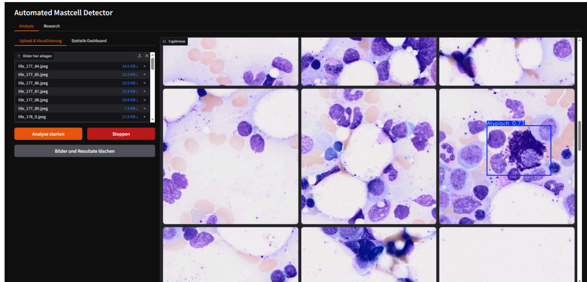
Figure 3: Analysis tab of the Gradio prototype showing uploaded image tiles with YOLO detection overlays.
