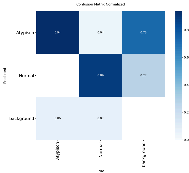
Figure 18: Normalized confusion matrix for P6-A (best.pt, evaluated on the val split). Rows are predicted classes; columns are ground-truth classes.
