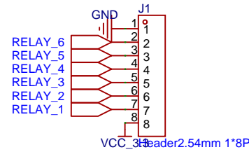
Relay module 6
