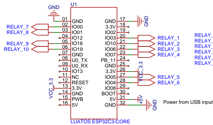
Relay module 6
