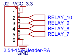
Relay module 4
