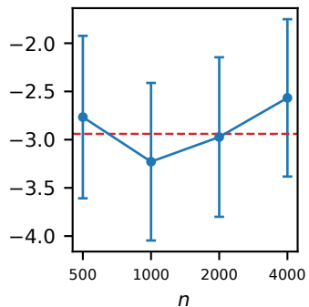
Gaussian, p=5
