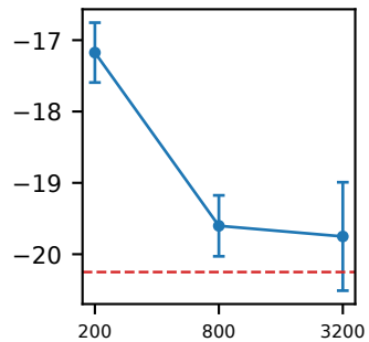
Gaussian, p=5
