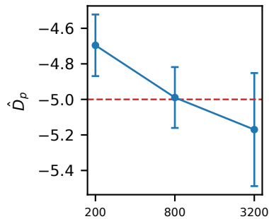
Mixed, het.
