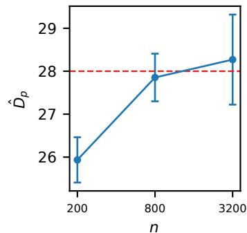
Mixed, het.
