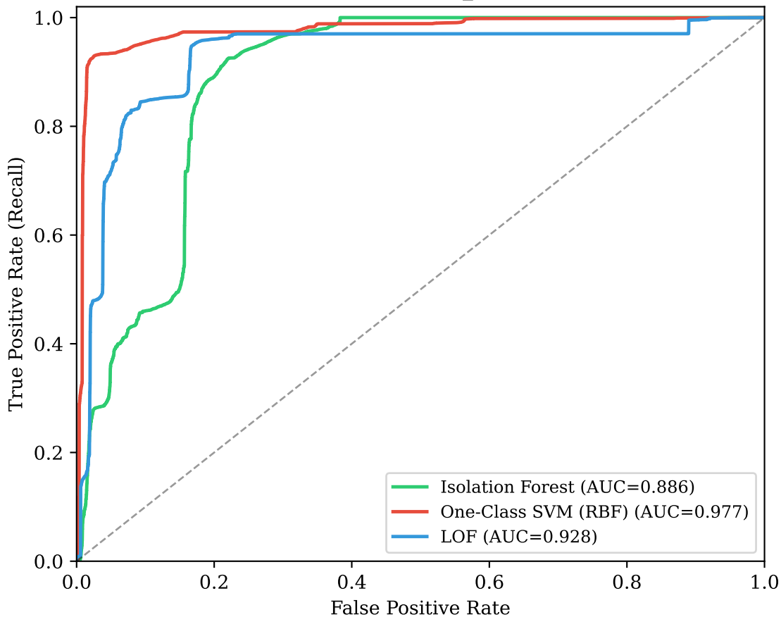
Stage-1 ROC Curves — TON_IoT (Validation Set)
