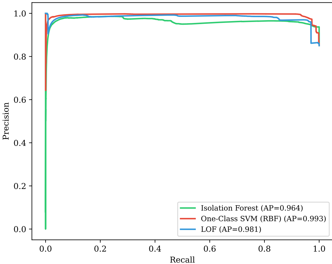
Stage-1 Precision-Recall Curves — TON_IoT (Validation Set)
