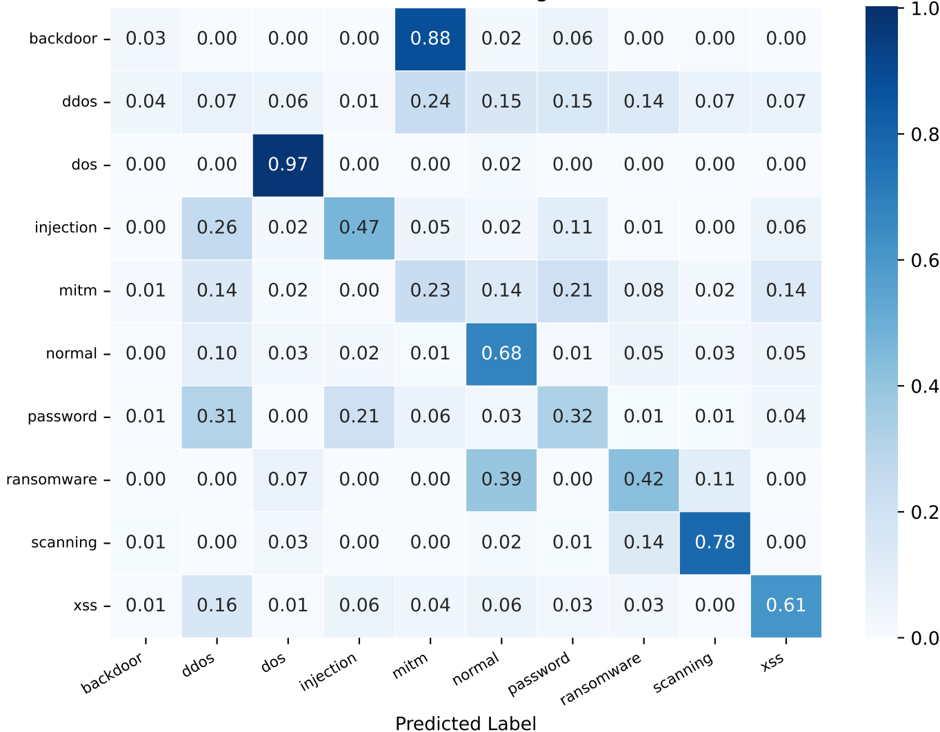
Normalized Confusion Matrix — LightGBM (standalone)
