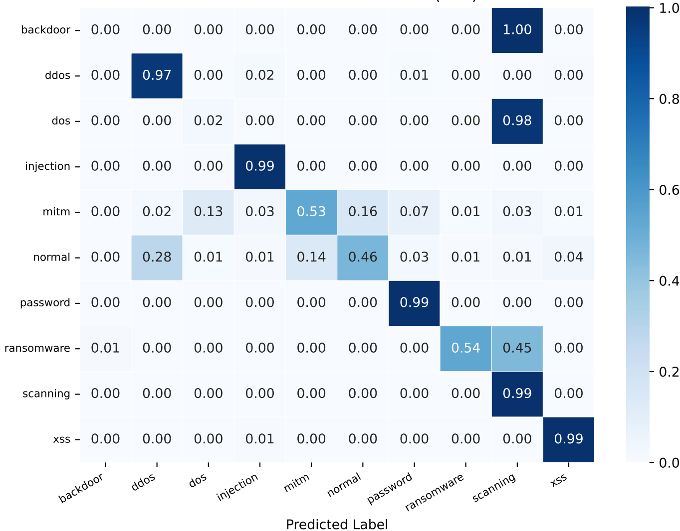
Normalized Confusion Matrix — One-Class SVM (RBF) + Random Forest
