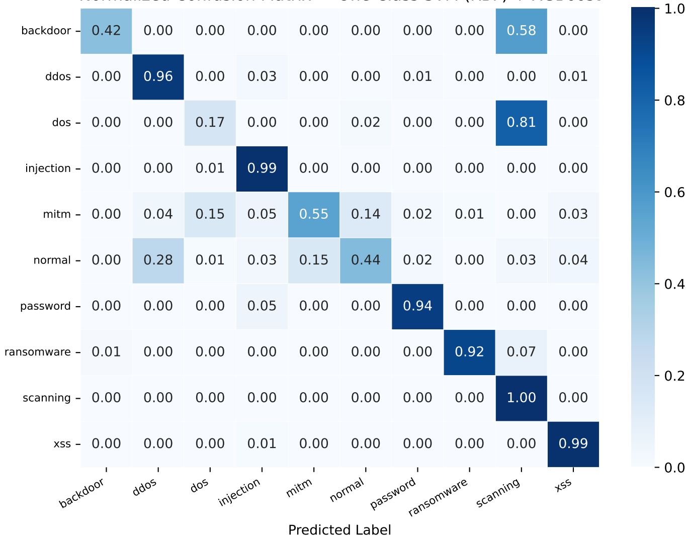
Normalized Confusion Matrix — One-Class SVM (RBF) + XGBoost
