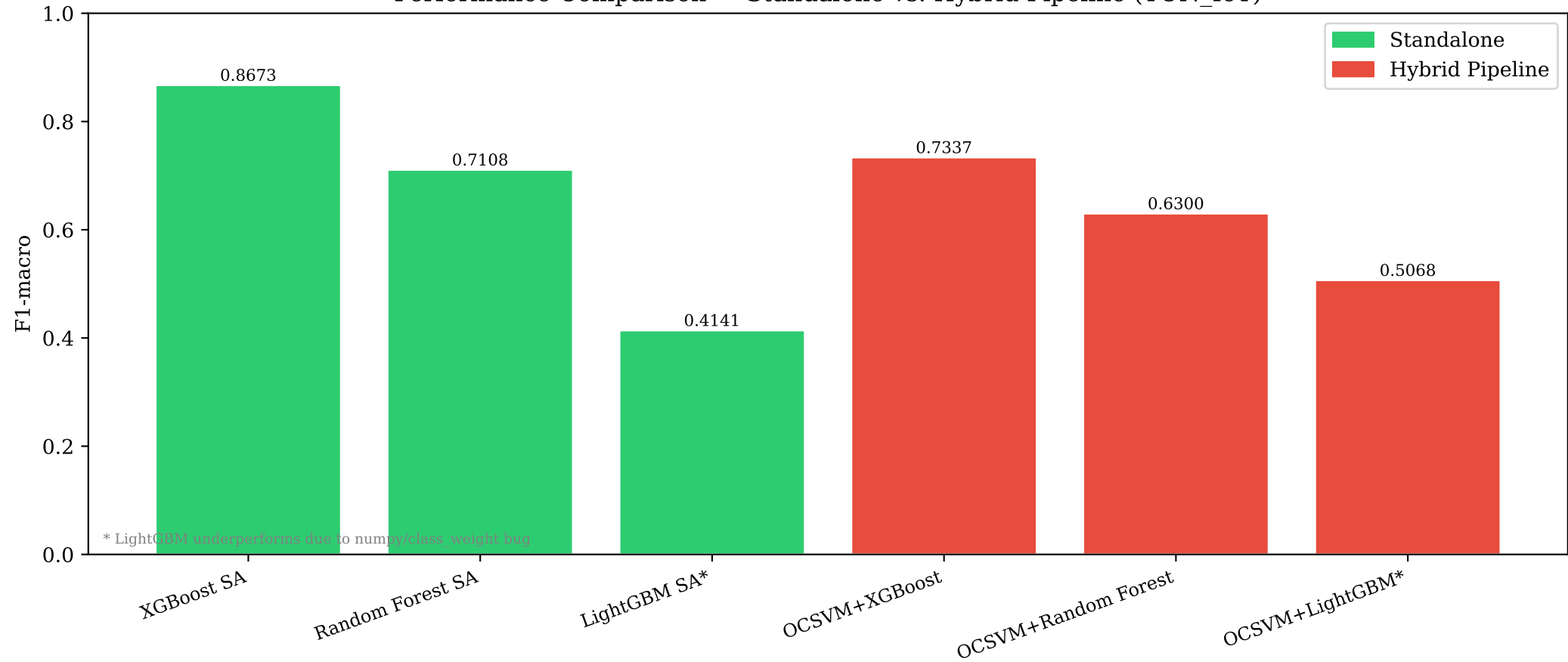
Performance Comparison — Standalone vs. Hybrid Pipeline (TON_IoT)
