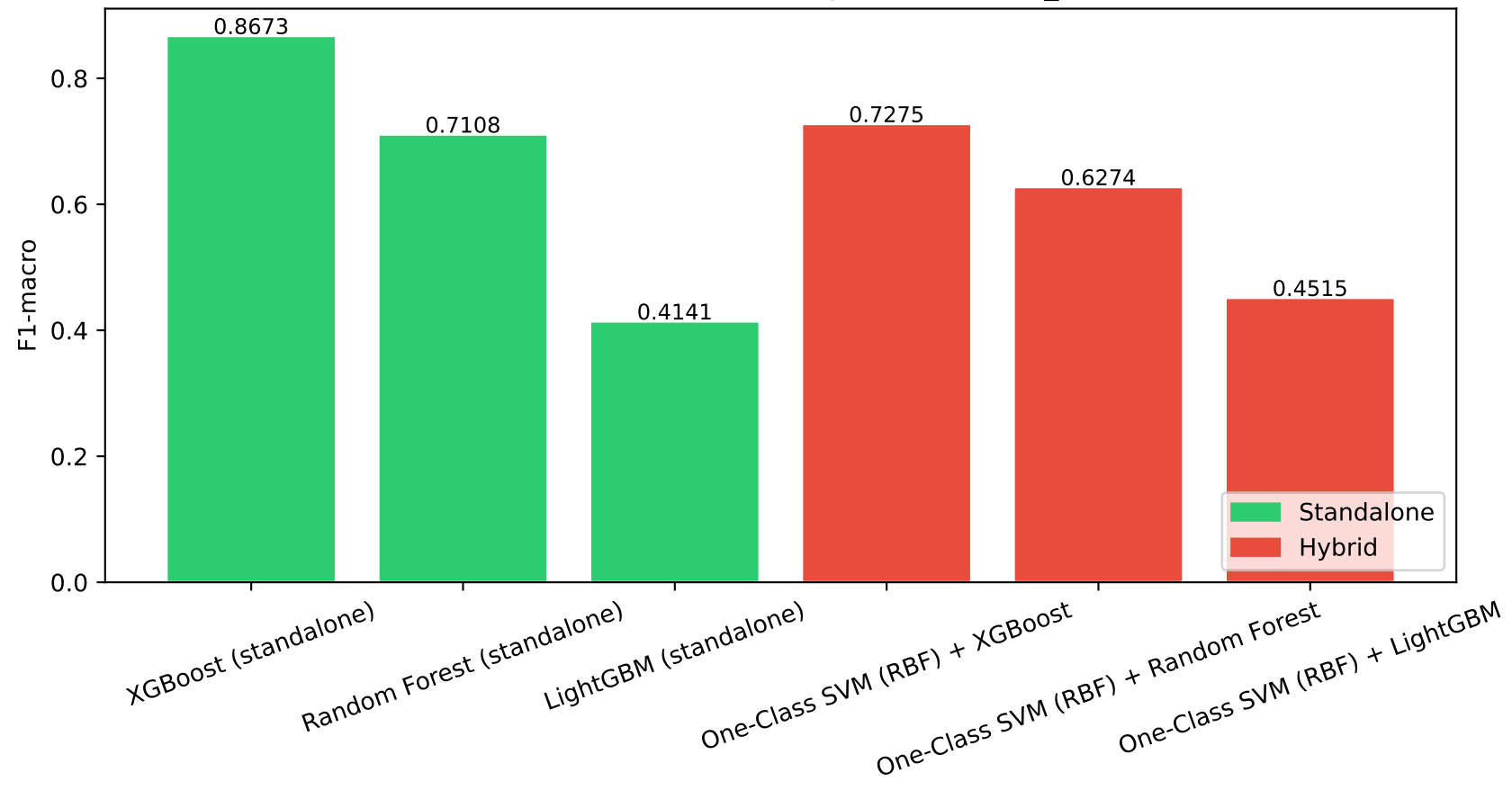
Overall Performance Comparison — TON_IoT
