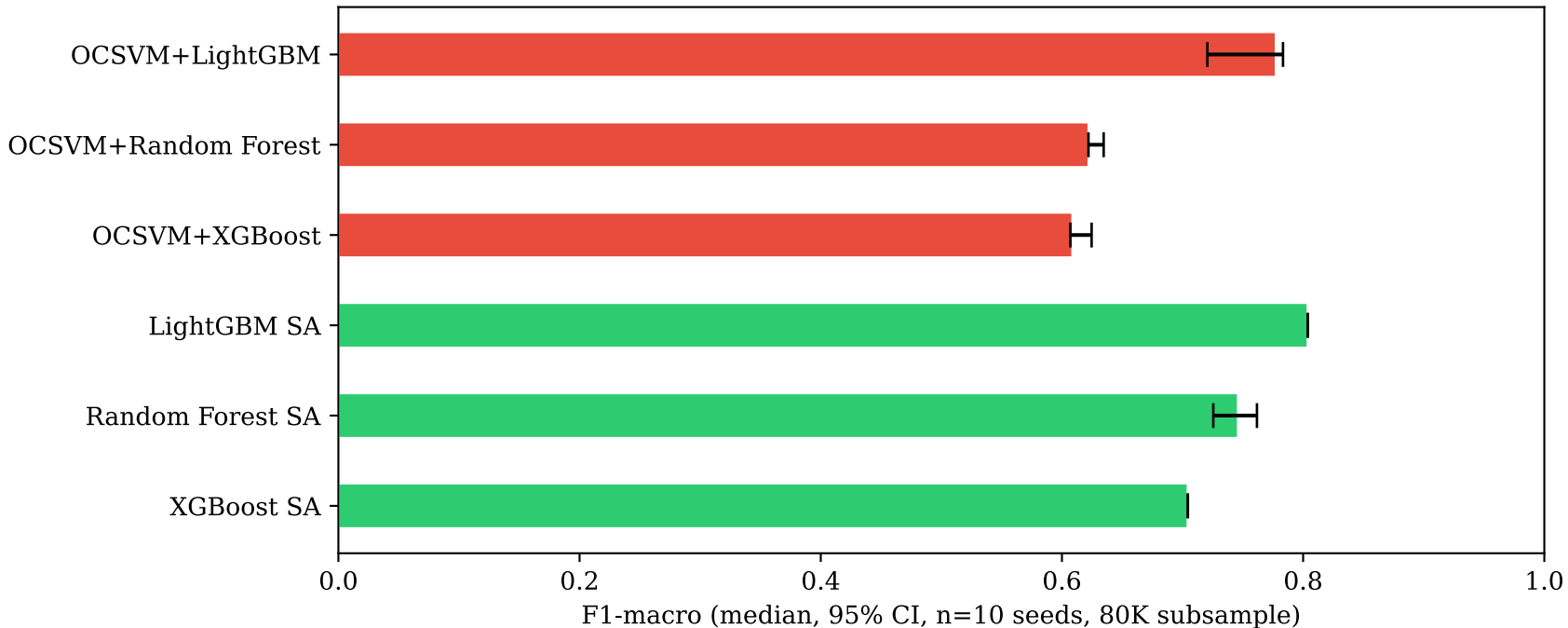
Bootstrap CI — Statistical Validation (TON_IoT)
