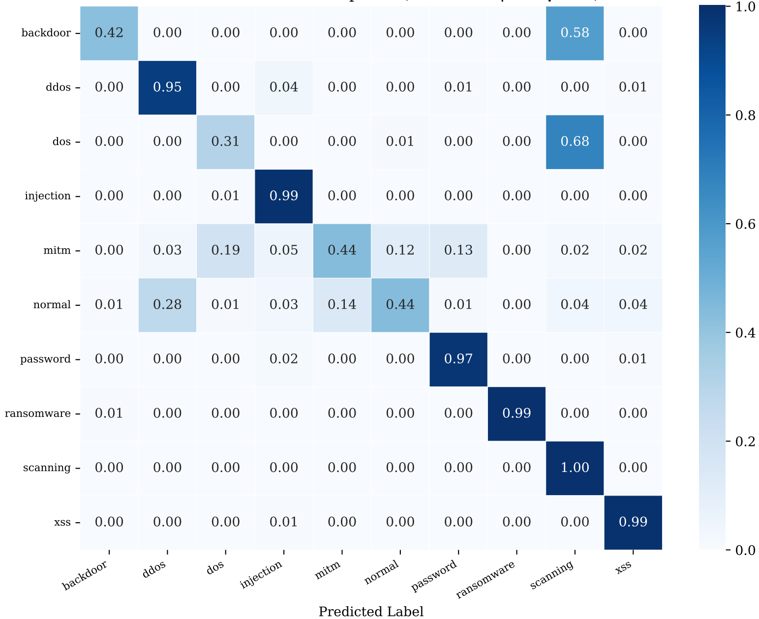
Normalized Confusion Matrix — Composite ( \alpha \cdot \text{OCSVM} + \beta \cdot \text{IF} + \gamma \cdot \text{LOF} ) + XGBoost
