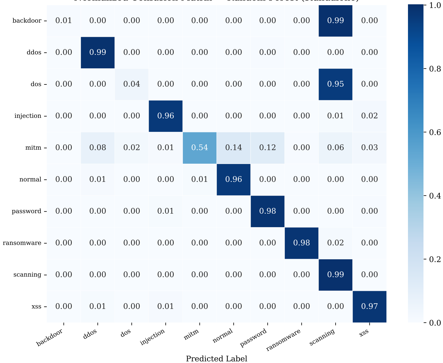
Normalized Confusion Matrix — Random Forest (standalone)
