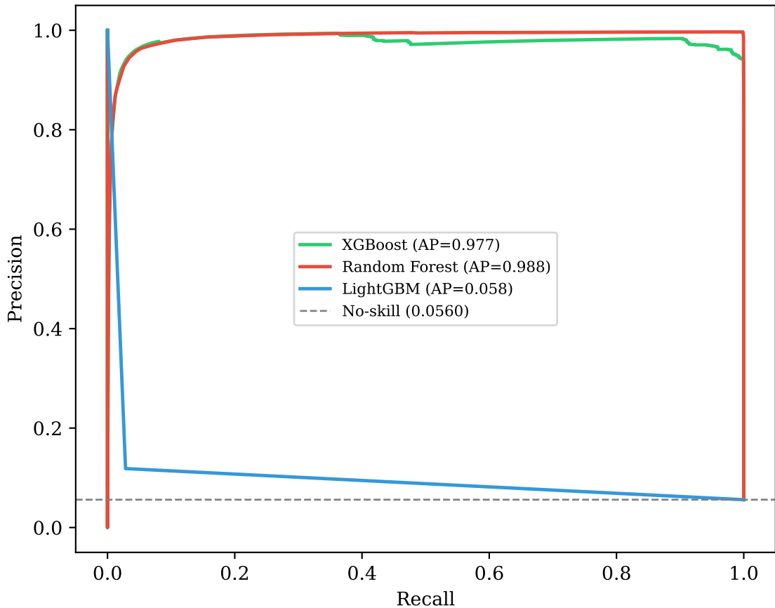
PR Curve — backdoor | T0807 (Command-Line Interface / Backdoor)
