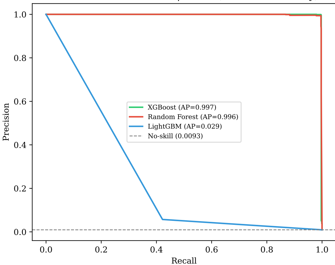
PR Curve — ransomware | T0826 (Loss of Availability)
