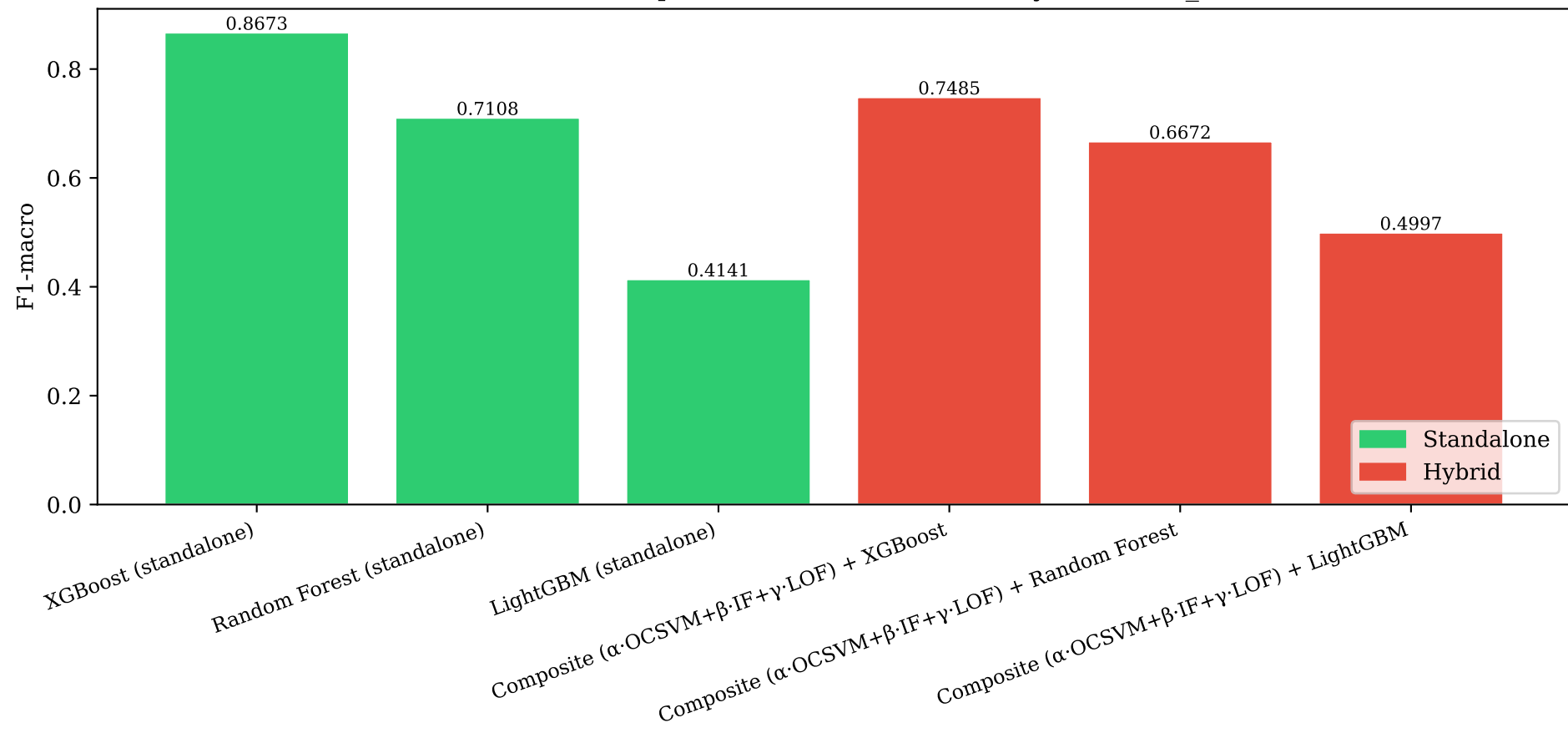
Performance Comparison — Standalone vs. Hybrid (TON_IoT)
