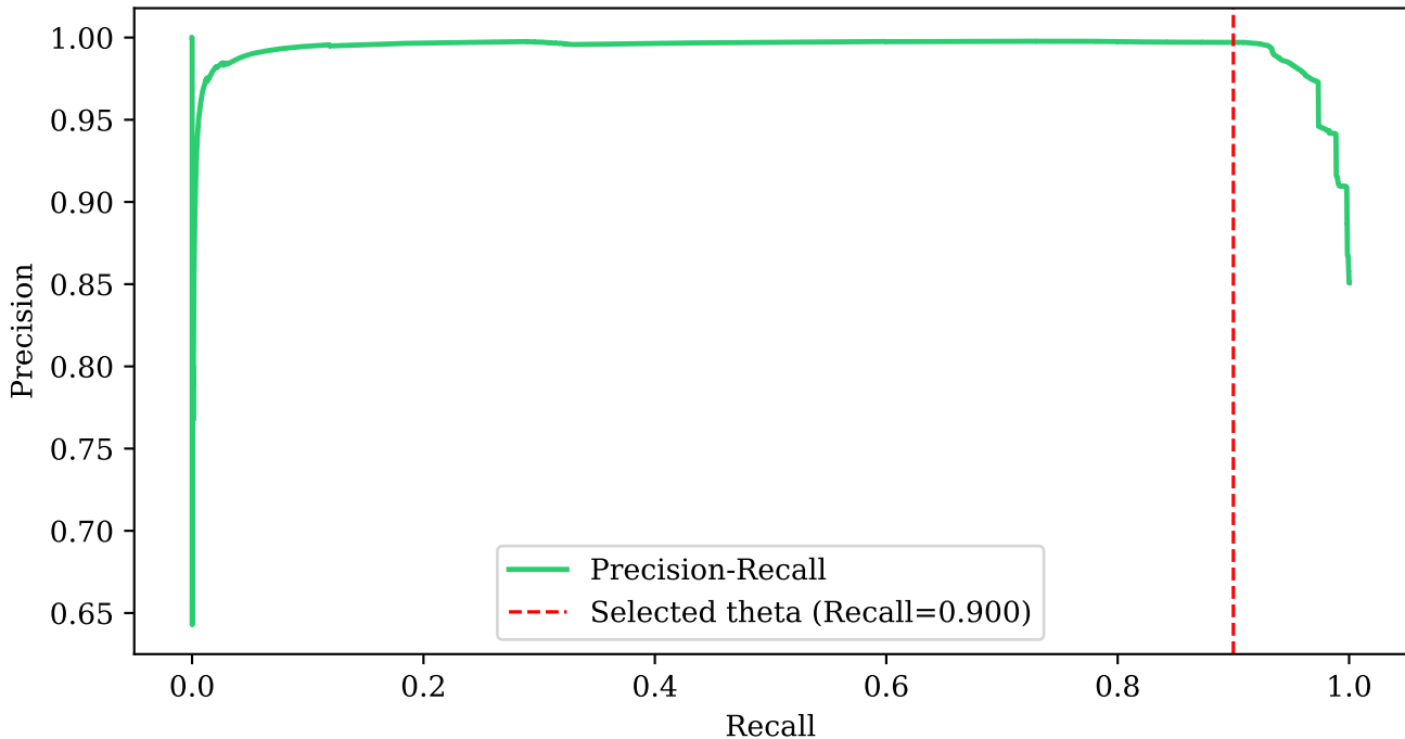
Threshold Calibration — One-Class SVM (RBF) (Validation Set)
