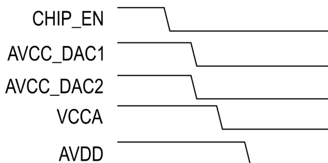
Figure 19 – Recommended Power Down Sequence
