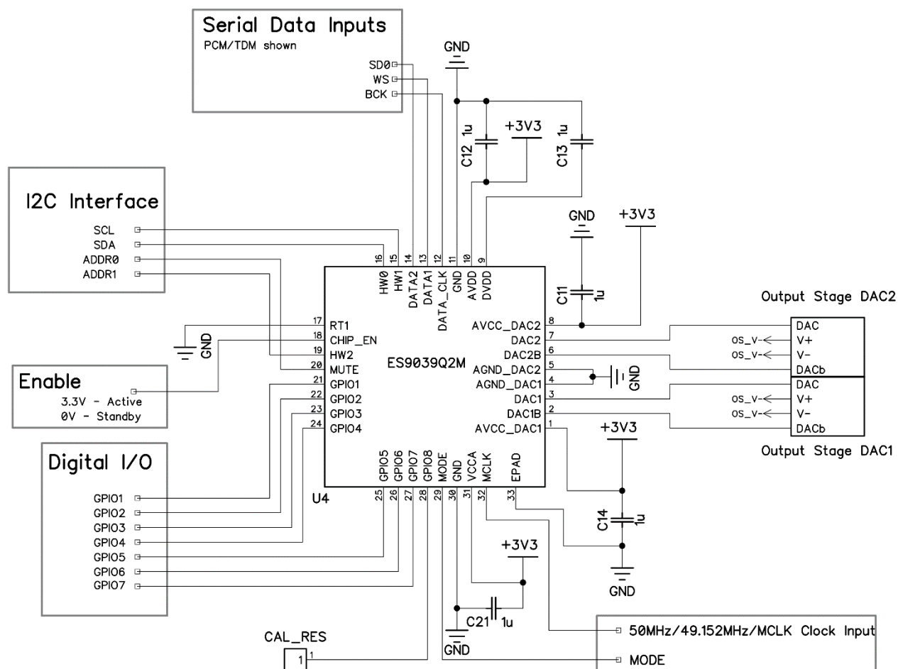
Figure 28 - Software Mode Reference Schematic for ES9039Q2M
