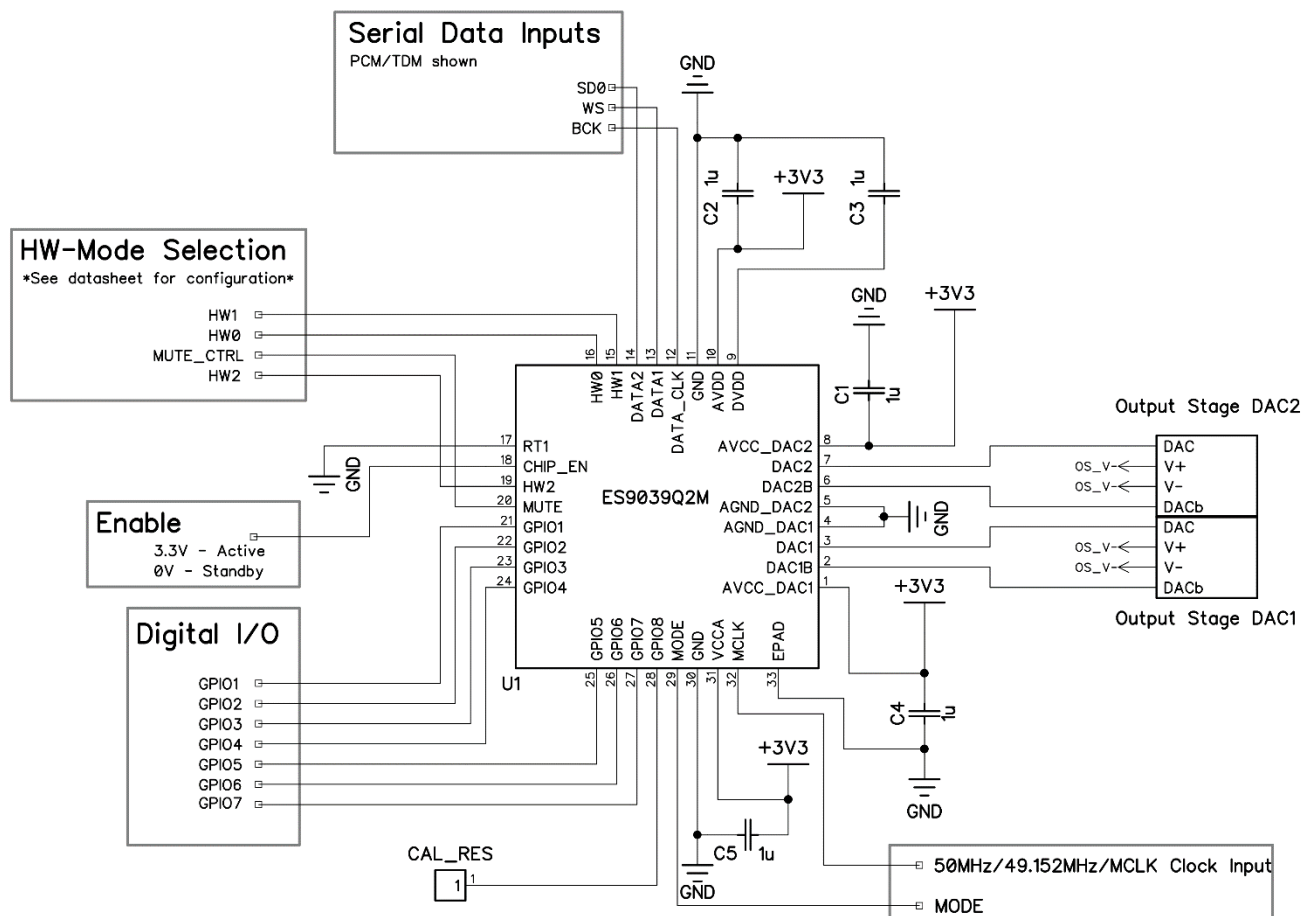
Figure 27 - Hardware (HW) Mode Reference Schematic for ES9039Q2M
