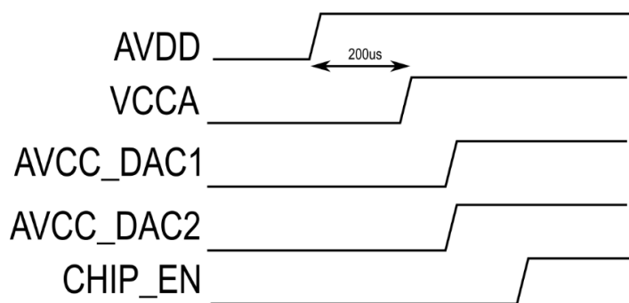
Figure 18 – Recommended Power Up Sequence
