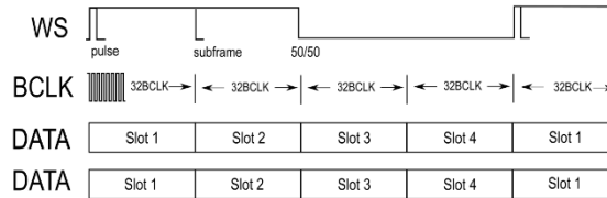
Figure 8 - TDM128 Mode
