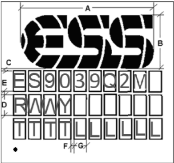
Figure 32 - ES9039Q2M Marking
