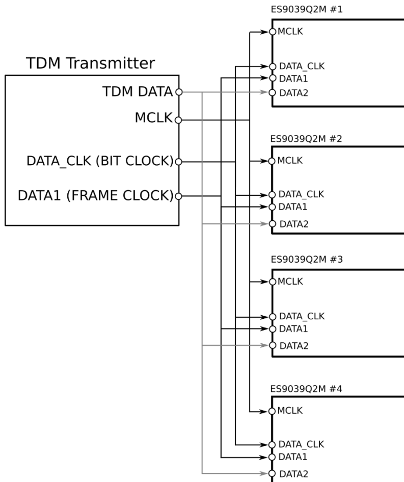
Figure 12 - TDM Connection of Several ES9039Q2M Devices in Parallel
