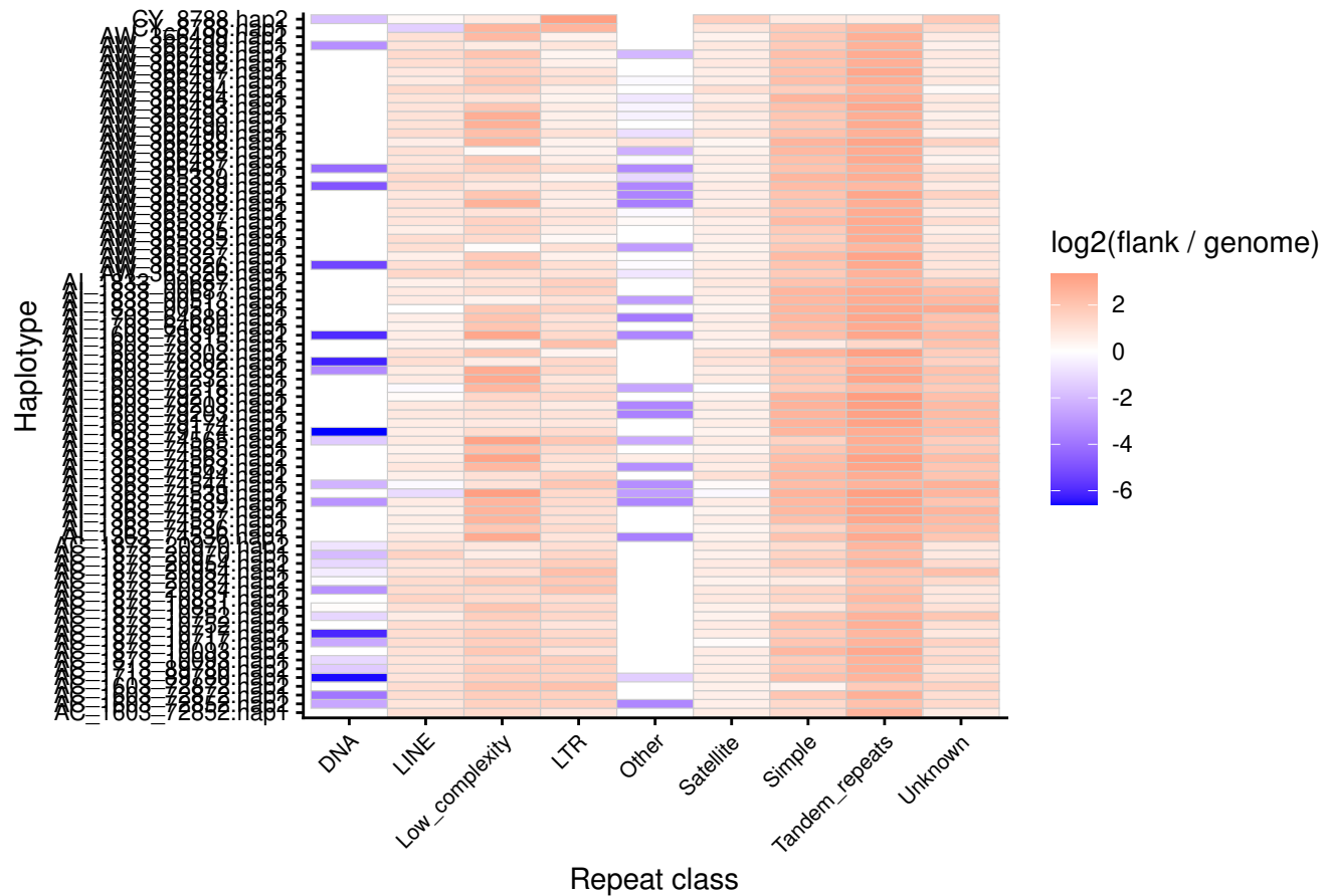
Scrub-jay: log2 enrichment of repeats in flanks around ROI (PAF-ba
