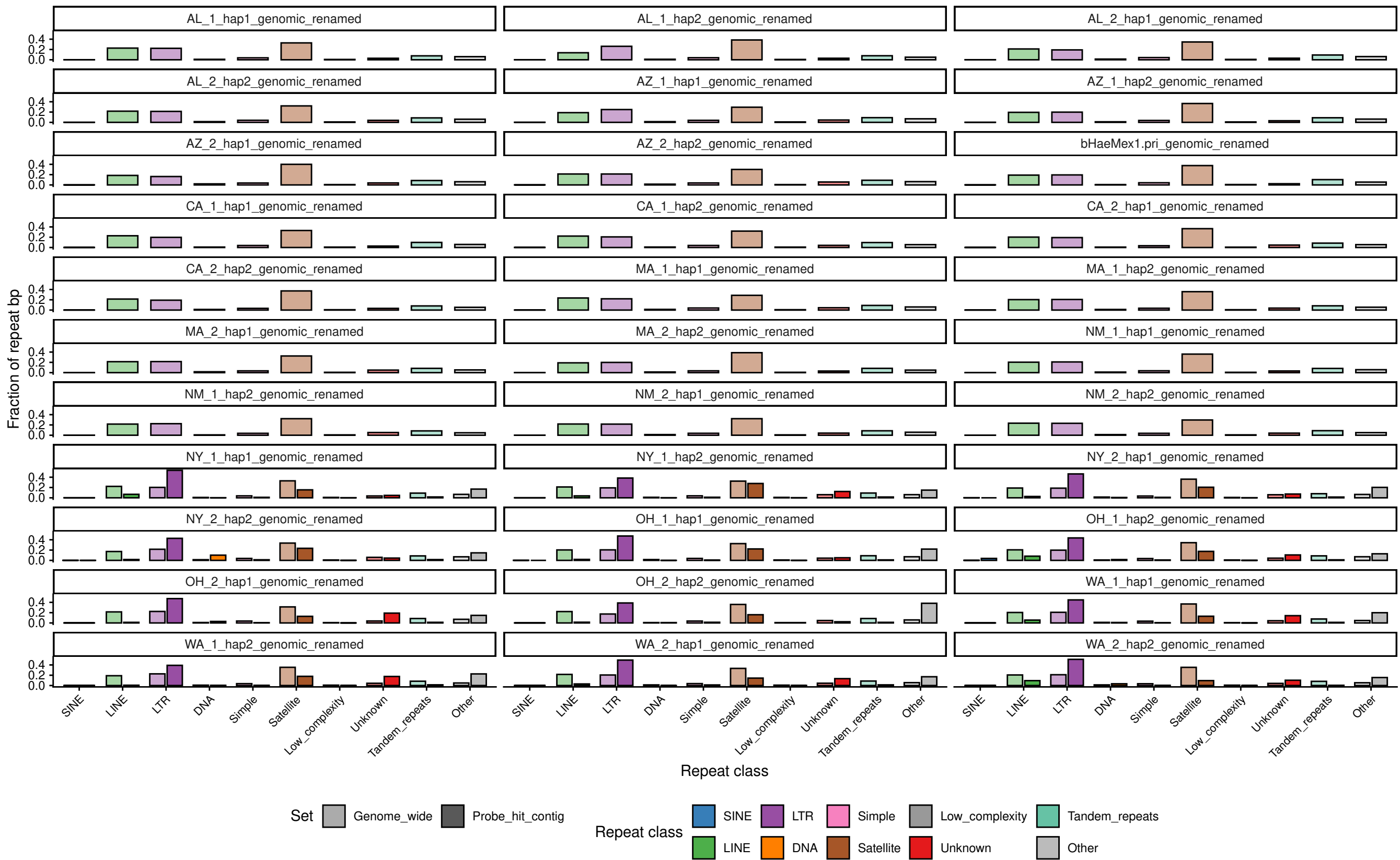
Genome-wide vs ROI contig repeat composition (HOPI, PAF-based)
