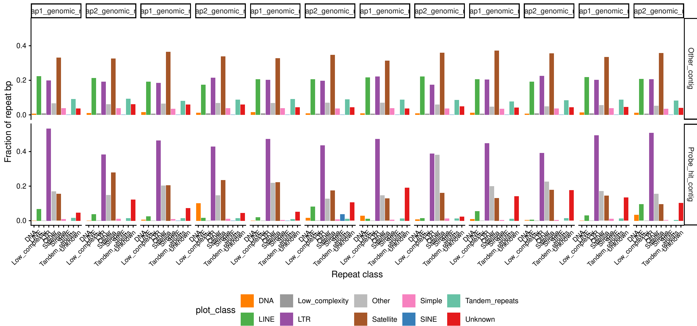
Repeat composition: ROI vs other contigs (HOFI, PAF-based)
