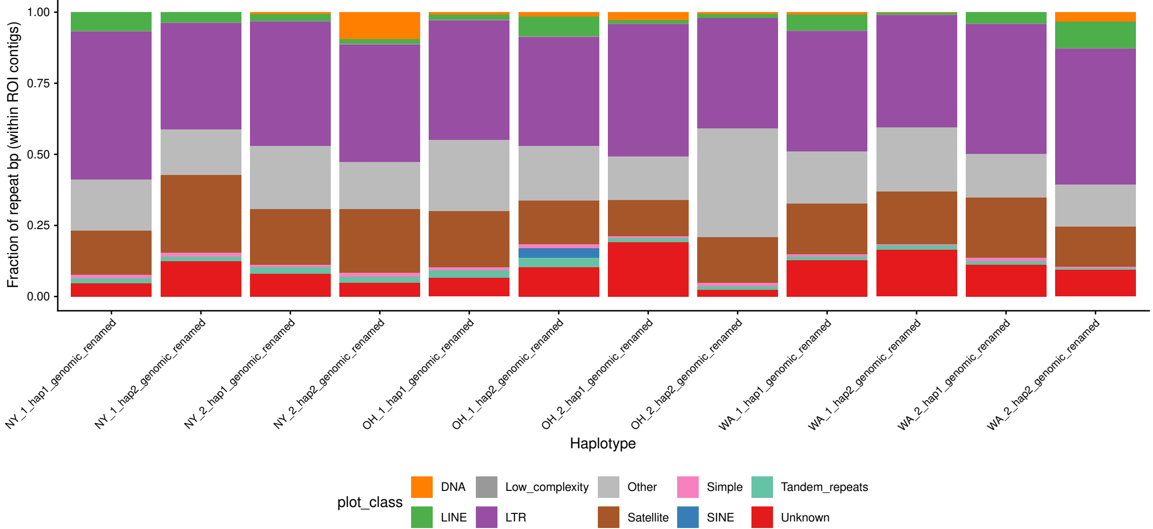
Repeat composition on ROI contigs (HOPI, PAF-based)
