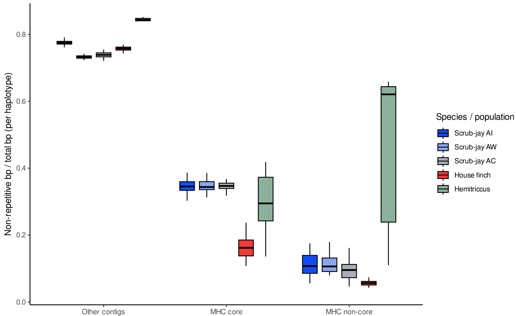
Non-repetitive fraction by contig type and species
