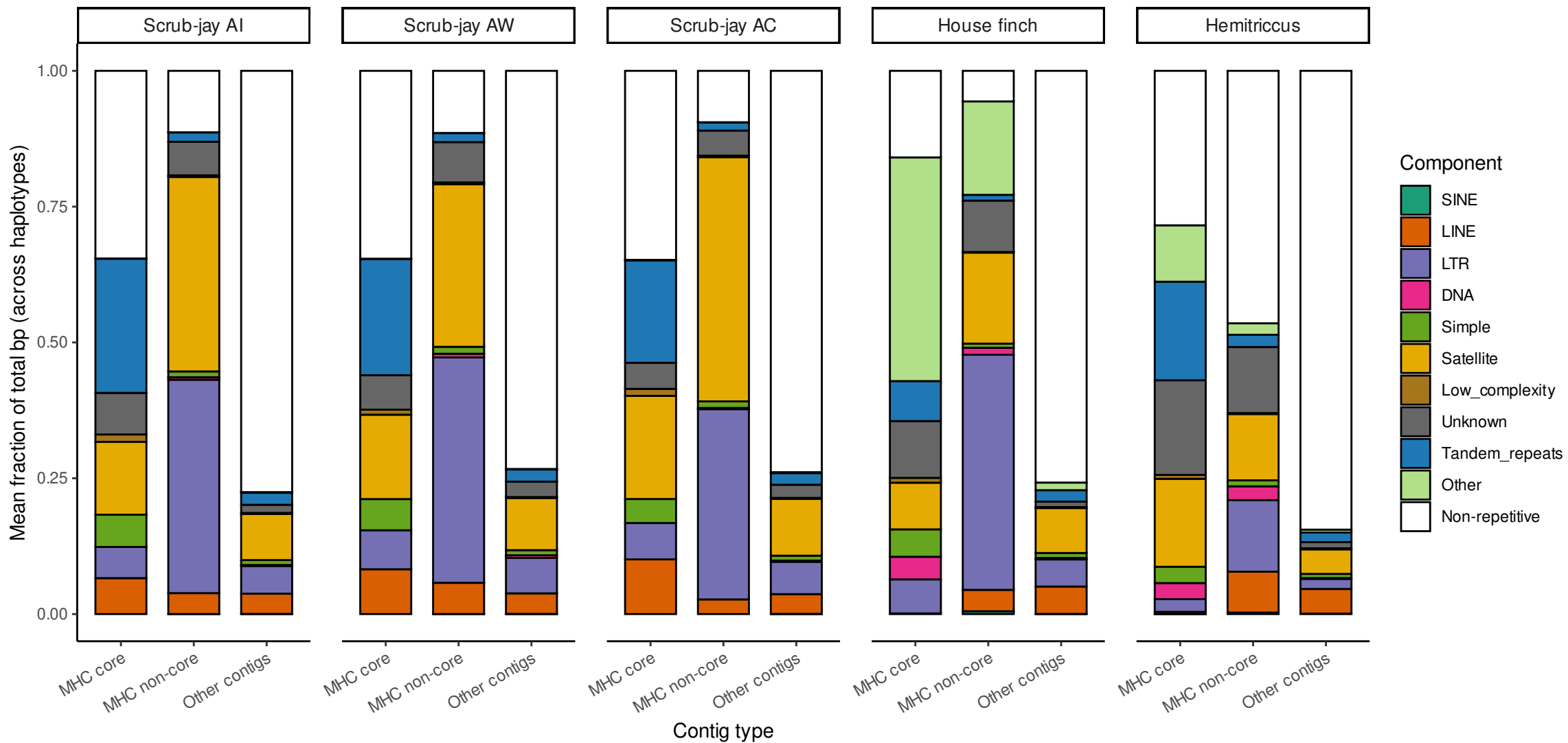
Repeat and non-repetitive composition by contig type across species
