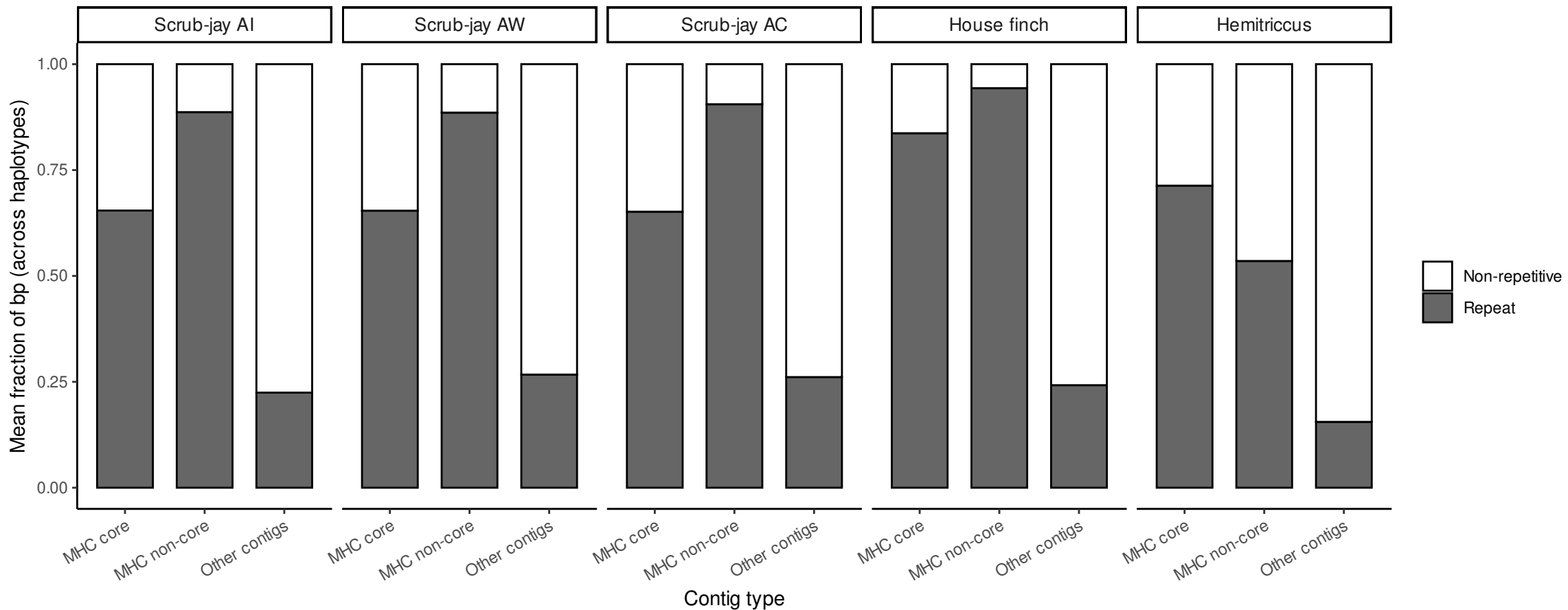
Repeat vs non-repetitive fraction by species and contig type
