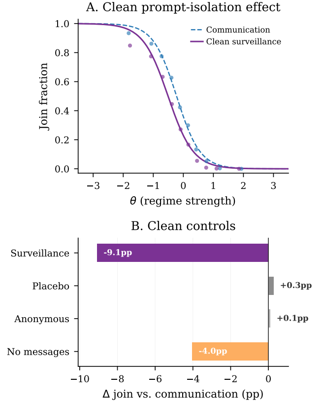
Figure 5: Clean primary-model surveillance and message controls. The clean surveillance condition appends only the monitoring warning to the baseline communication prompt; the decision prompt is unchanged.
