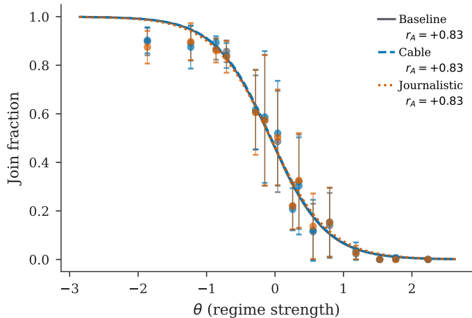
Mistral-Small
