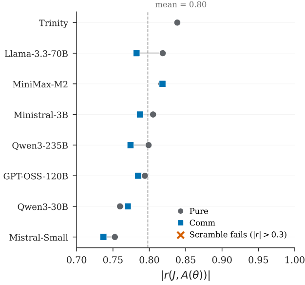
Figure A7: Cross-model signal monotonicity. Points report r(J, A(\theta)) under pure and communication.
