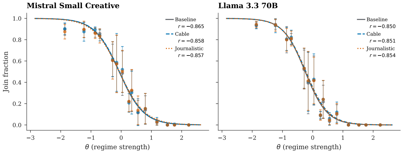
Figure A6: Cross-generator robustness. Three text formats produce indistinguishable sigmoids.
