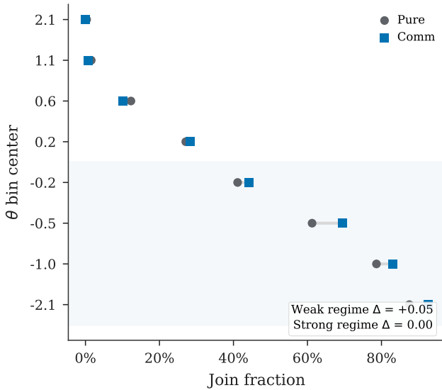
Figure 4: Communication effect by regime strength, pooled across 7 models.
