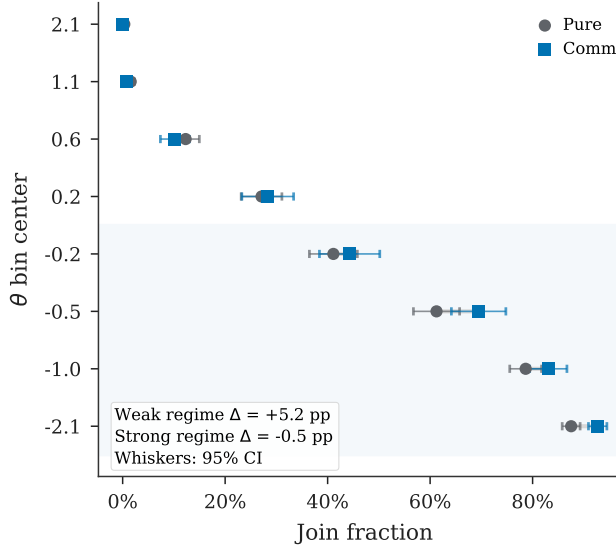
Figure 4: Communication effect by regime strength, pooled across 7 models. Points are mean join rates by \theta bin under the pure and communication treatments; whiskers are 95% confidence intervals on bin means; the shaded region marks weak-regime states ( \theta < 0 ). In-figure \Delta annotations are in percentage points.
