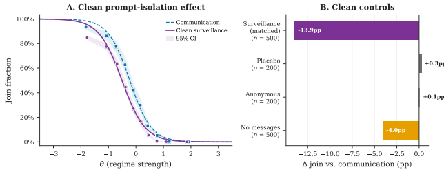
Figure 5: Clean primary-model surveillance and message controls (Mistral). Panel A : Join curves under communication baseline vs. clean surveillance; shaded bands are 95% confidence intervals; surveillance shifts the curve downward while preserving threshold structure. Panel B : The clean-surveillance bar uses the matched-cell estimator ( n = 500 matched cells); placebo ( n = 200 ), anonymous ( n = 200 ), and no-message ( n = 500 ) bars are control deltas against the main communication baseline; per-bar sample sizes appear on the axis labels, and inference is reported in Tables A9 and A10. Placebo and anonymous monitoring warnings sit near zero.
