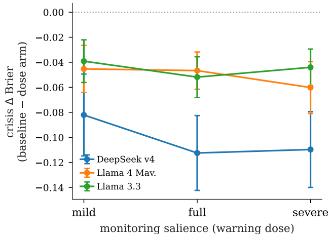
(b) Blinding: already near-maximal at mild
