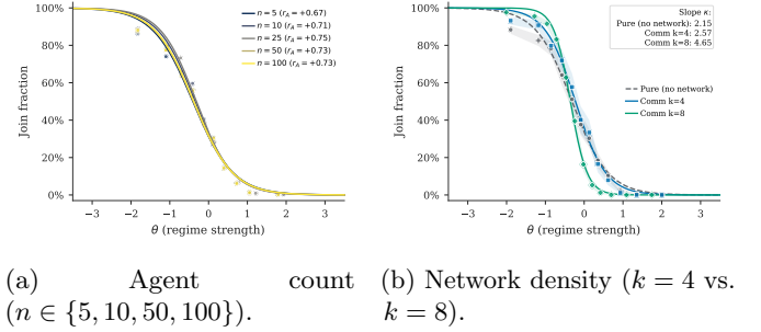
Figure A4: Robustness checks for threshold-policy alignment (Mistral). Points are period-level join fractions with fitted logistic curves. In panel (a), legend entries report r(J, A(\theta)) per agent count; in panel (b), the inset reports fitted logistic slopes \kappa and shaded bands are 95% confidence intervals.
