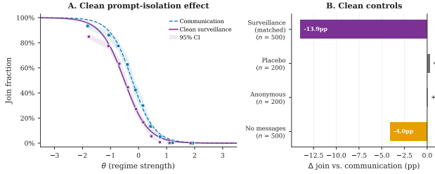
Figure 5: Clean primary-model surveillance and message controls (Mistral). Panel A : Join curves under communication baseline vs. clean surveillance; shaded bands are 95% confidence intervals; surveillance shifts the curve downward while preserving threshold structure. Panel B : The clean-surveillance bar uses the matched-cell estimator ( n = 500 matched cells); placebo ( n = 200 ), anonymous ( n = 200 ), and no-message ( n = 500 ) bars are control deltas against the main communication baseline; per-bar sample sizes appear on the axis labels, and inference is reported in Tables A9 and A10. Placebo and anonymous monitoring warnings sit near zero.
