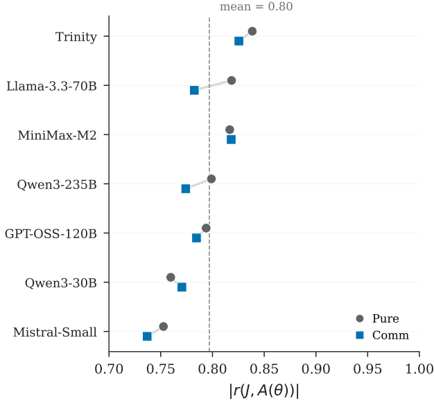
Figure A7: Cross-model signal monotonicity. Points report |r(J, A(\theta))| under pure and communication for each of the seven models; near-identical pure/communication pairs are vertically offset for visibility. Period-level samples per model and treatment are listed in Table A20.
