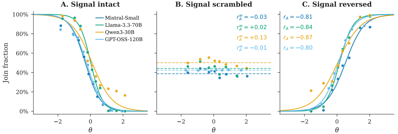
Figure 3: Falsification triptych. Plotted series show four representative model families; reported mean correlations are across all 7 models in Table 2, with per-arm period counts in Table A20. Left : Pure (mean r = +0.80 , raw per-model). Center : Scramble ( r = +0.03 , within-country). Right : Flip ( r = -0.80 ).
