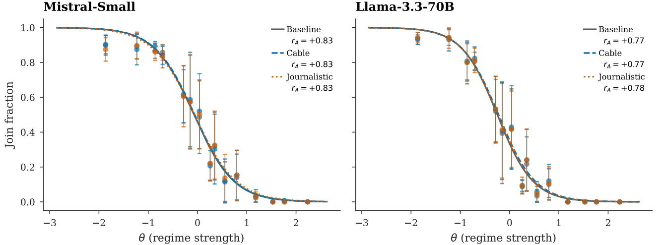
Figure A6: Cross-generator robustness (Mistral-Small and Llama-3.3-70B, pure treatment, N = 100 country-periods per format). Three text formats produce indistinguishable sigmoids; error bars are 95% confidence intervals on binned join rates. Legend correlations use the threshold-policy convention r(J, A(\theta)) and match Table A14.
