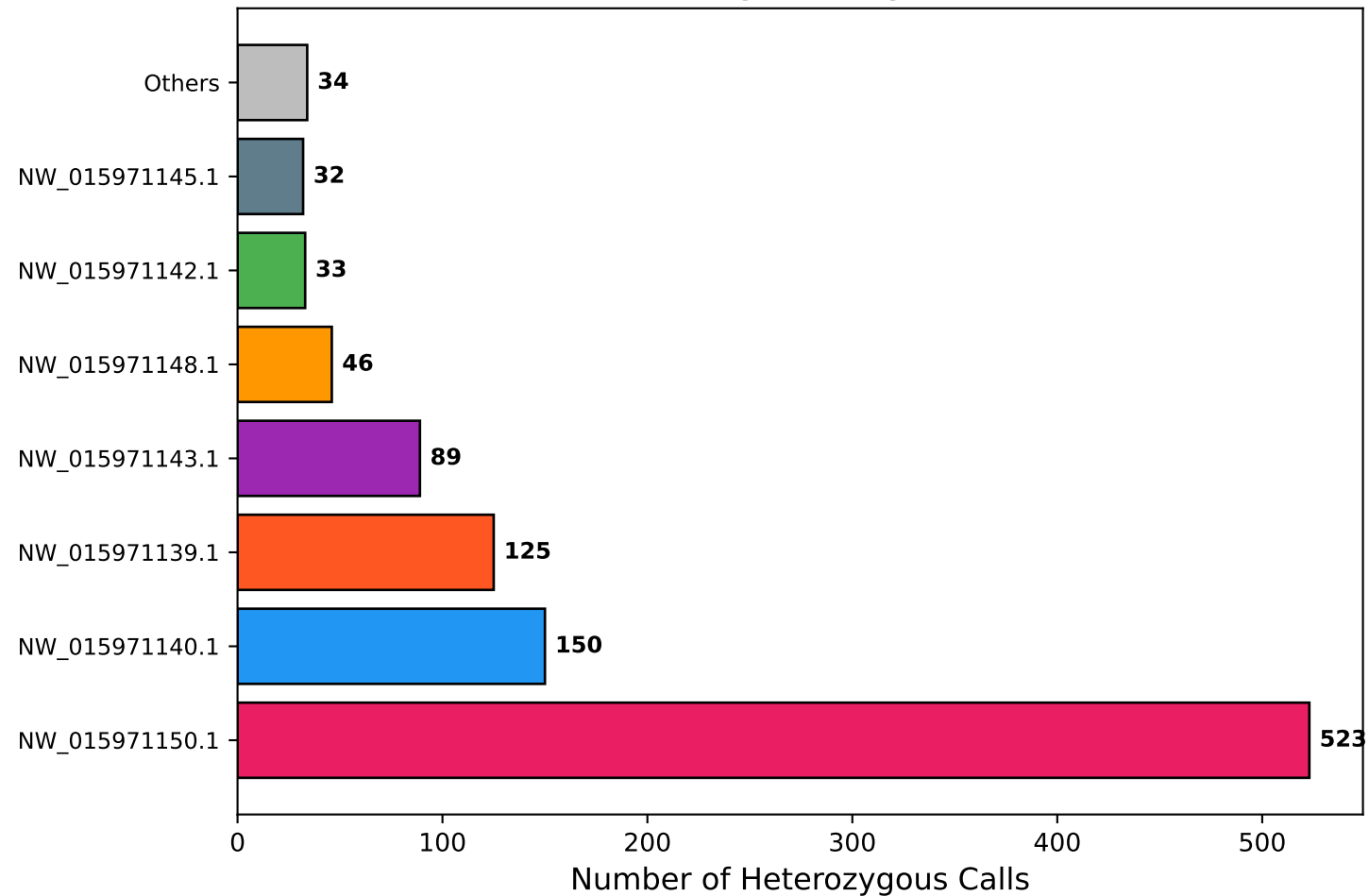
B. Heterozygous Call Distribution (Paralogous Regions)
