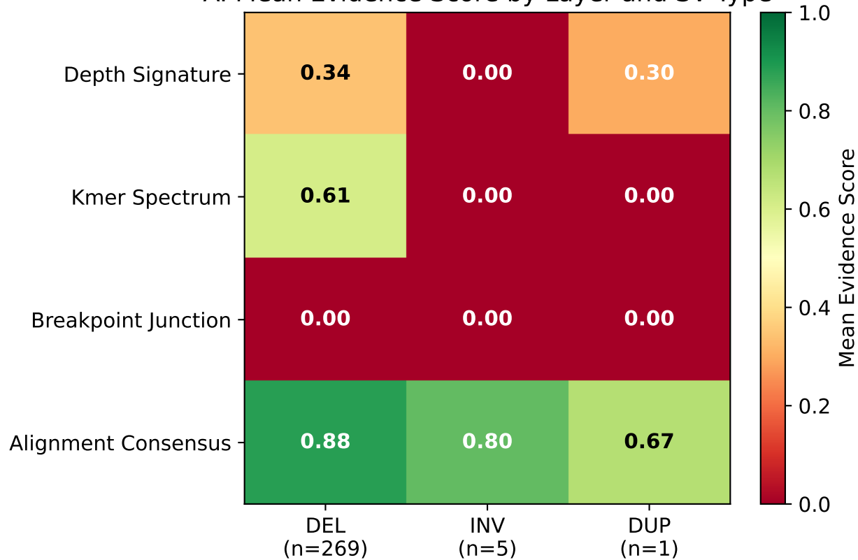
A. Mean Evidence Score by Layer and SV Type
