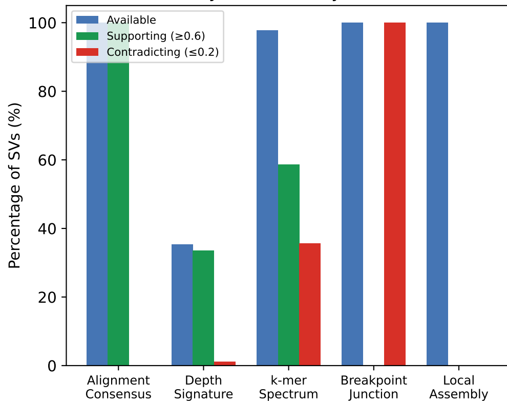
B. Evidence Layer Availability and Performance
