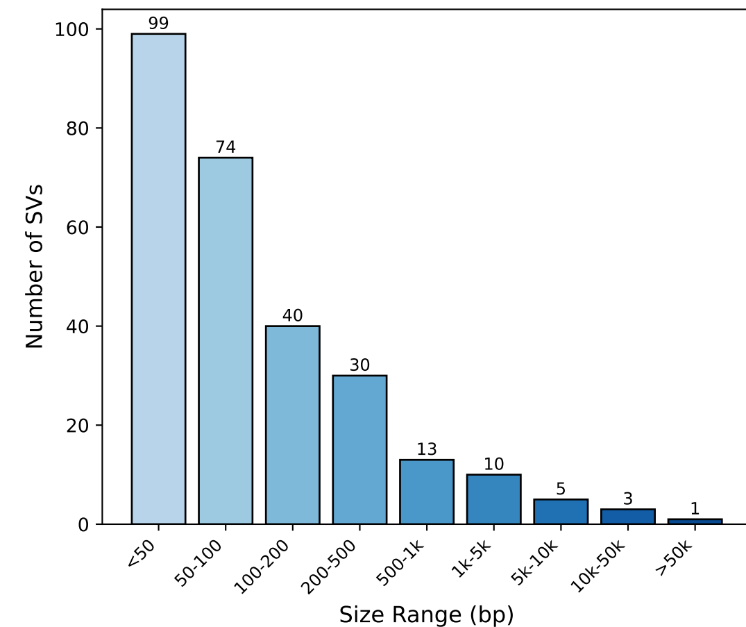
C. Consensus SV Size Distribution
