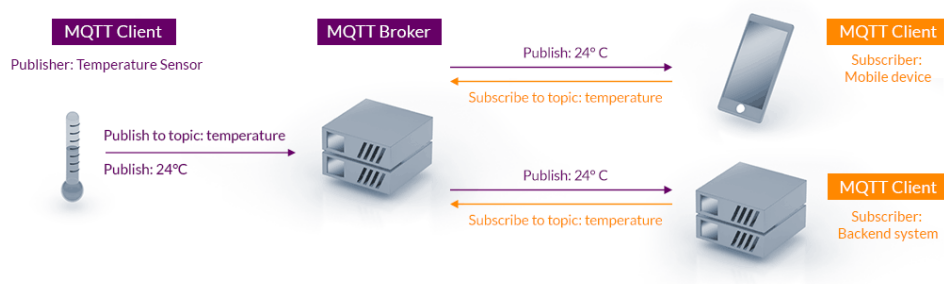
图 1.1: MQTT Publish / Subscribe Architecture
