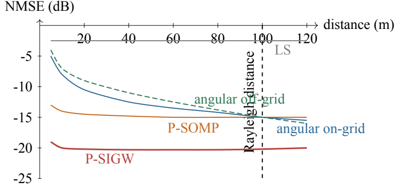
Figure 7: Trend-focused redraw of NMSE versus distance from [1, Fig. 10].
