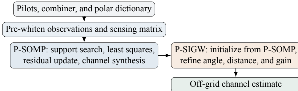
Figure 6: Combined workflow of the P-SOMP and P-SIGW algorithms.
