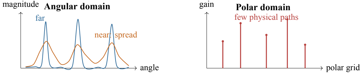
Figure 2: Energy spread and polar sparsity, adapted from Figs. 2 and 8 of [1].
