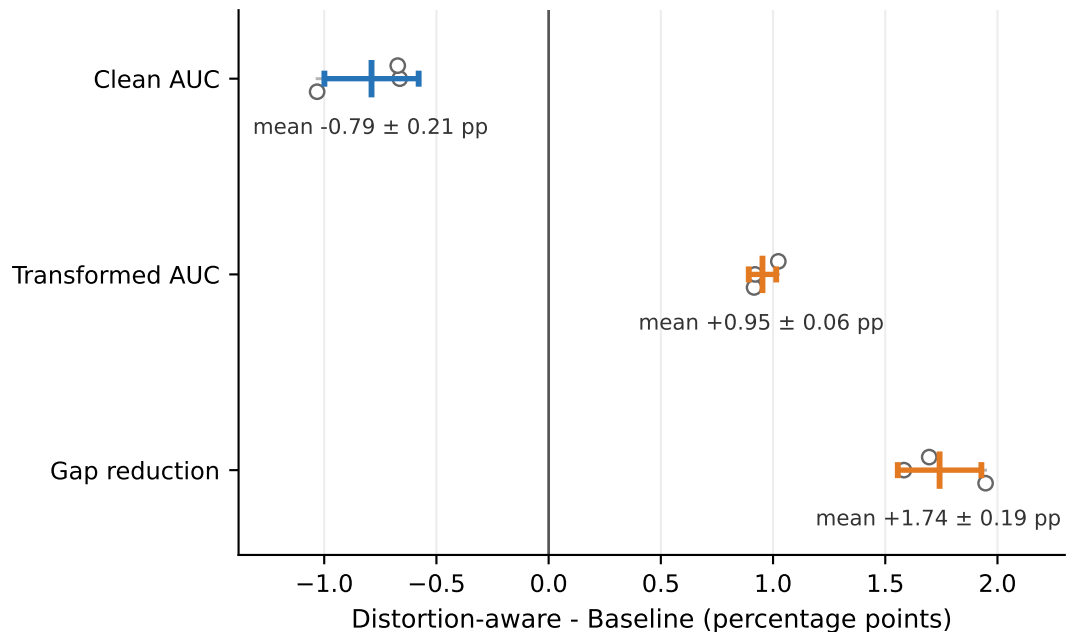
Paired effects for individual seeds
