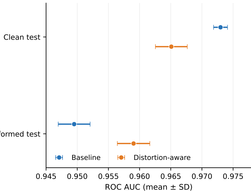
Performance across three seeds
