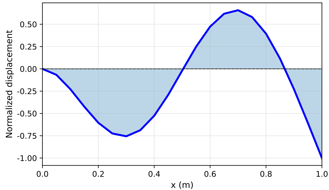
Mode 3: f_3 = 293.23 Hz
