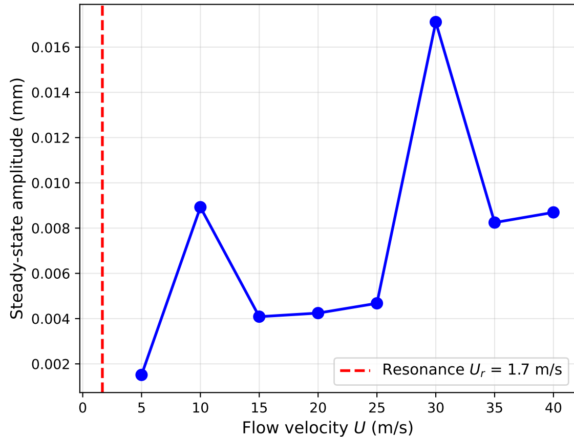
Vortex-Induced Vibration: Amplitude vs Velocity
