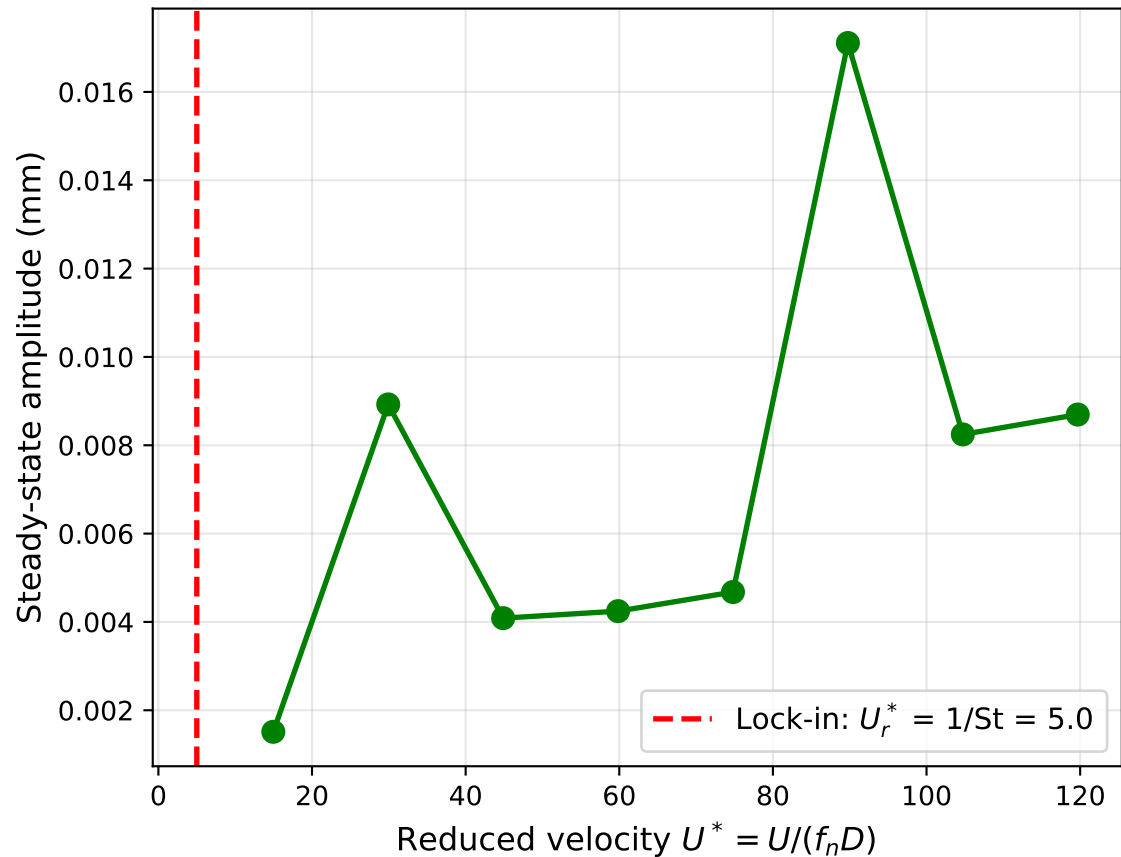
Response in Terms of Reduced Velocity
