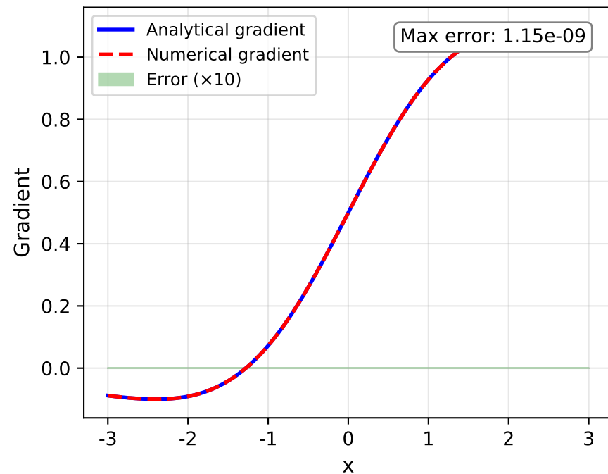
Swish: Gradient Verification
