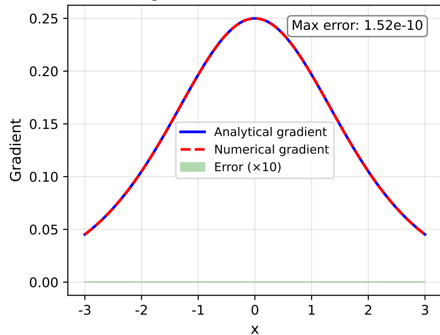
Sigmoid: Gradient Verification
