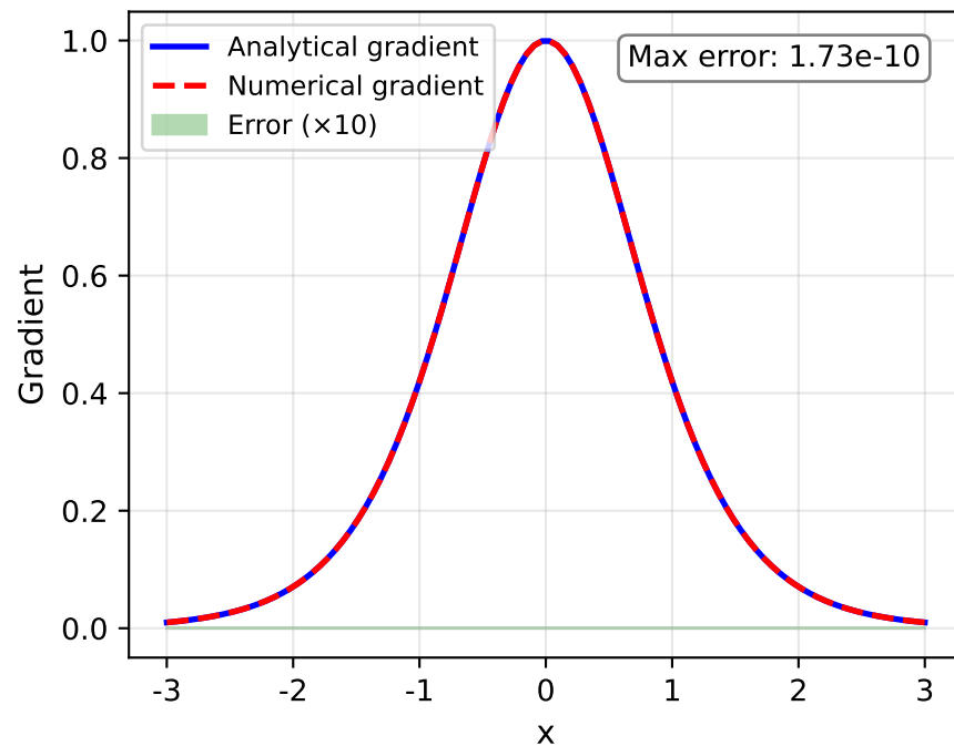
Tanh: Gradient Verification
