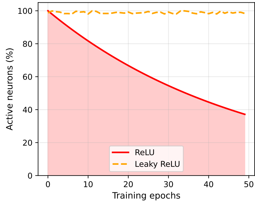
Dead ReLU Problem
