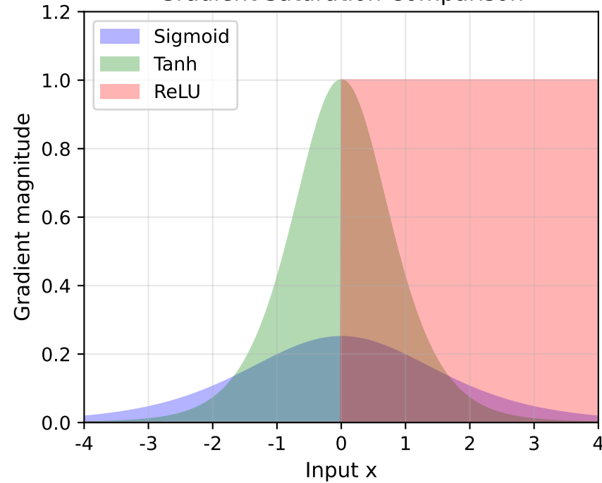
Gradient Saturation Comparison
