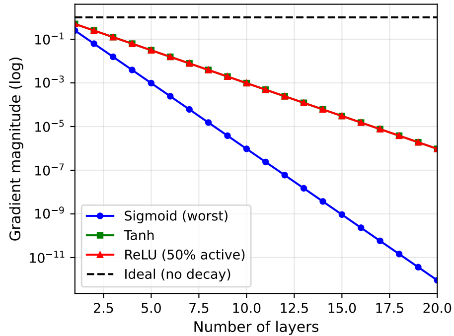
Vanishing Gradient Problem
