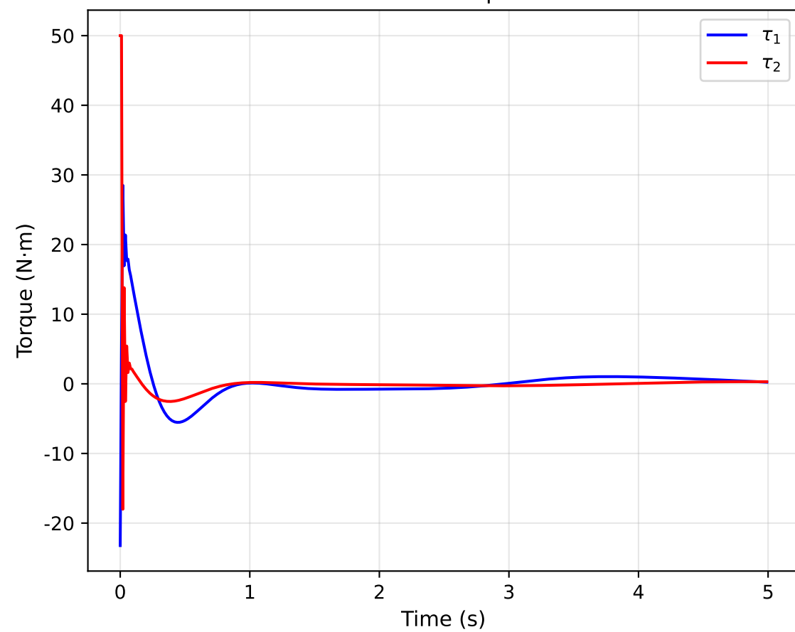
Control Torques
