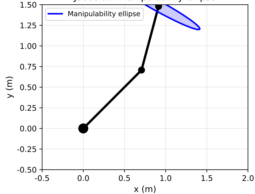
Jacobian: Manipulability Ellipse
