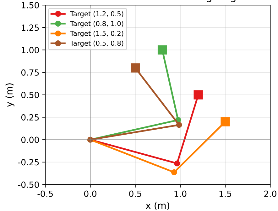
Inverse Kinematics: Reaching Targets
