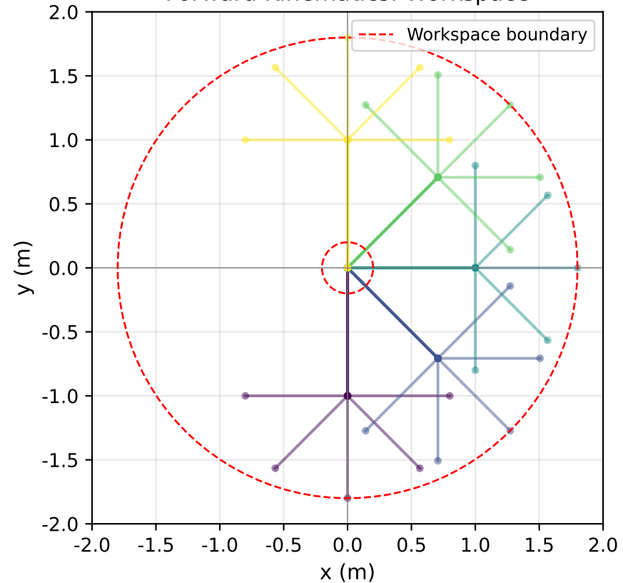
Forward Kinematics: Workspace
